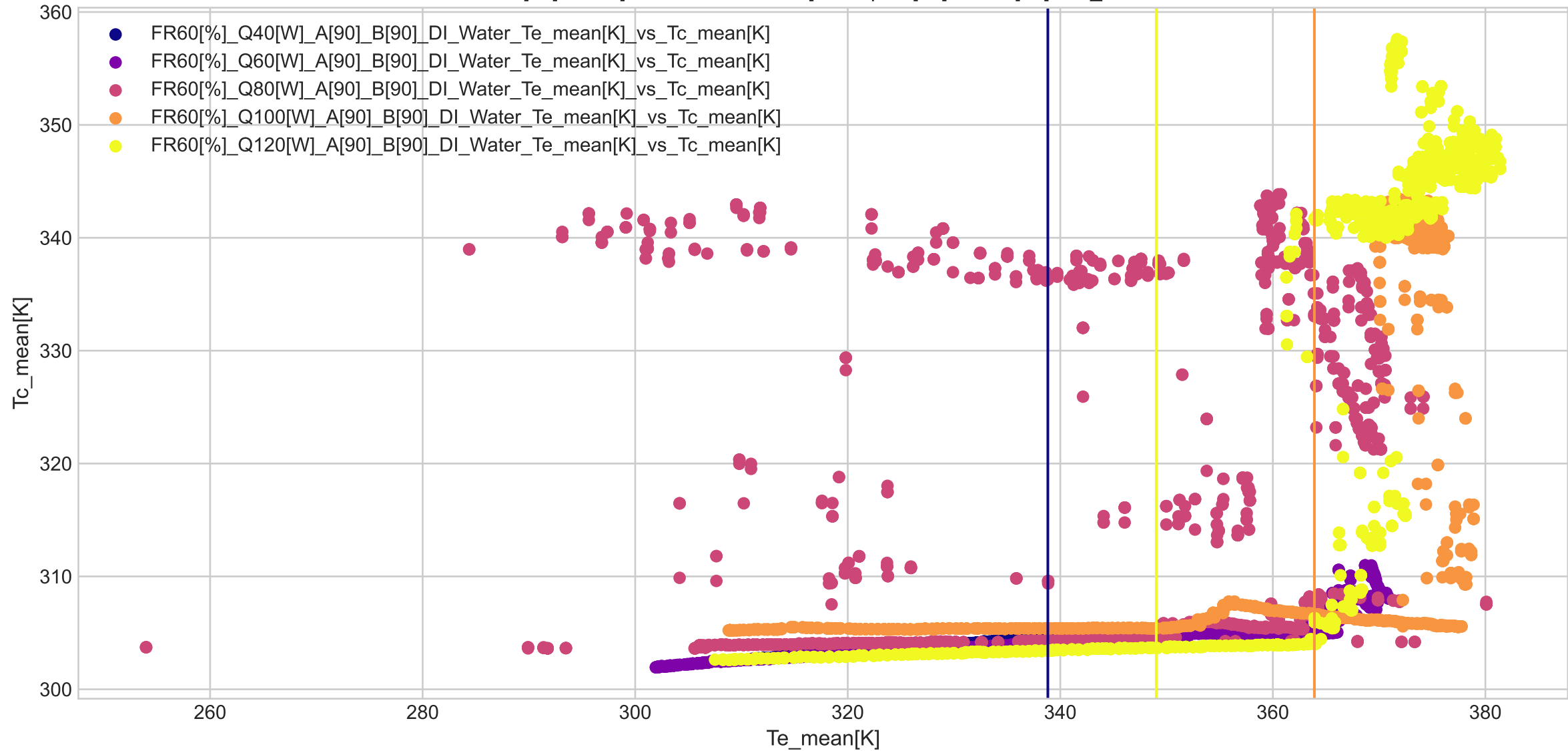
FR [60]% - Q [ 40 60 80 100 120]W - alpha [90] - beta [90] - DI_Water
